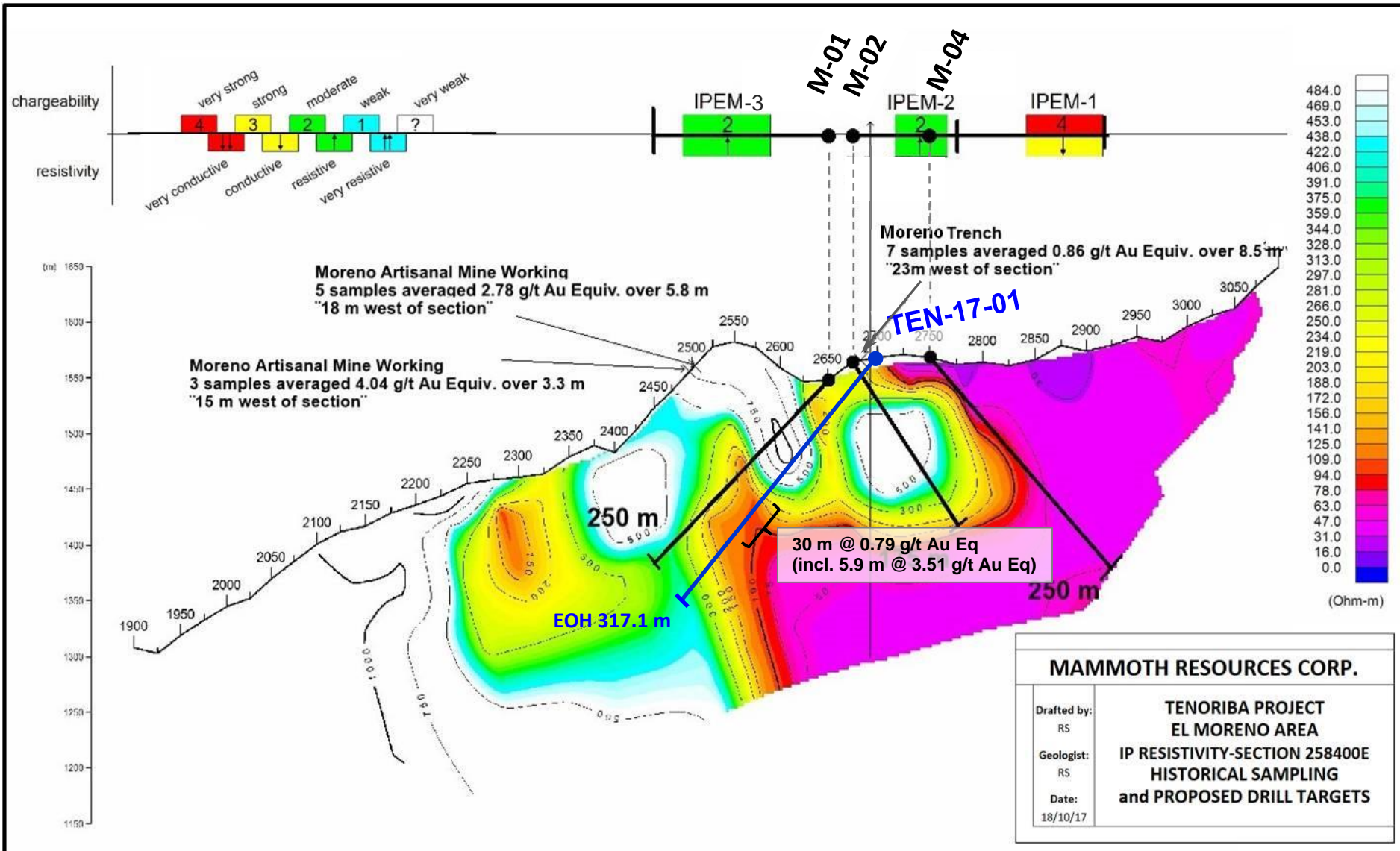
Figure 2 - TEN-17-01 location and gold interval relative to geophysical features and proposed hole locations M-01, M-02 & M-04
