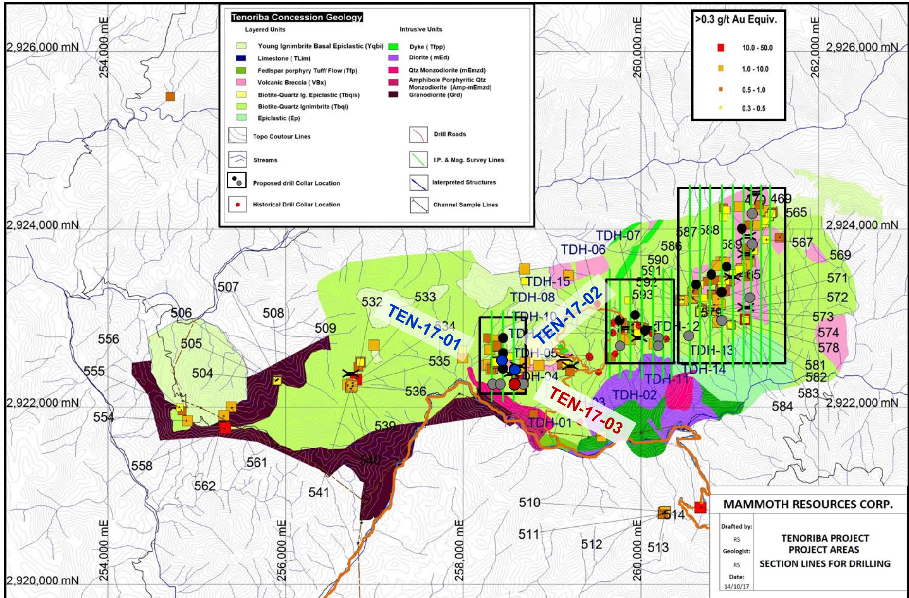
Figure 1 - Surface Map, Tenoriba Property, Proposed and Actual Drill Hole Locations
