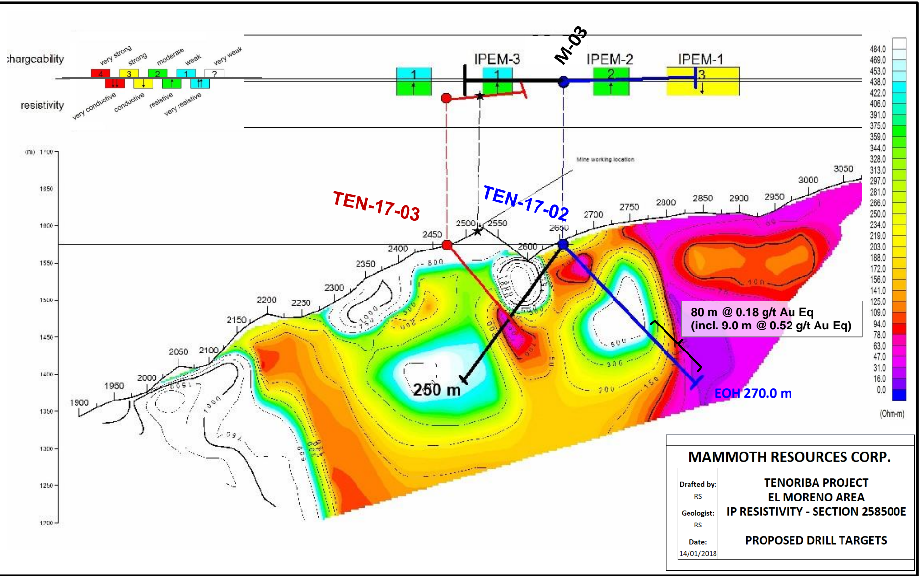
Figure 3 - TEN-17-02 location and gold interval relative to geophysical features and proposed hole locations TEN-17-03 and M-03
